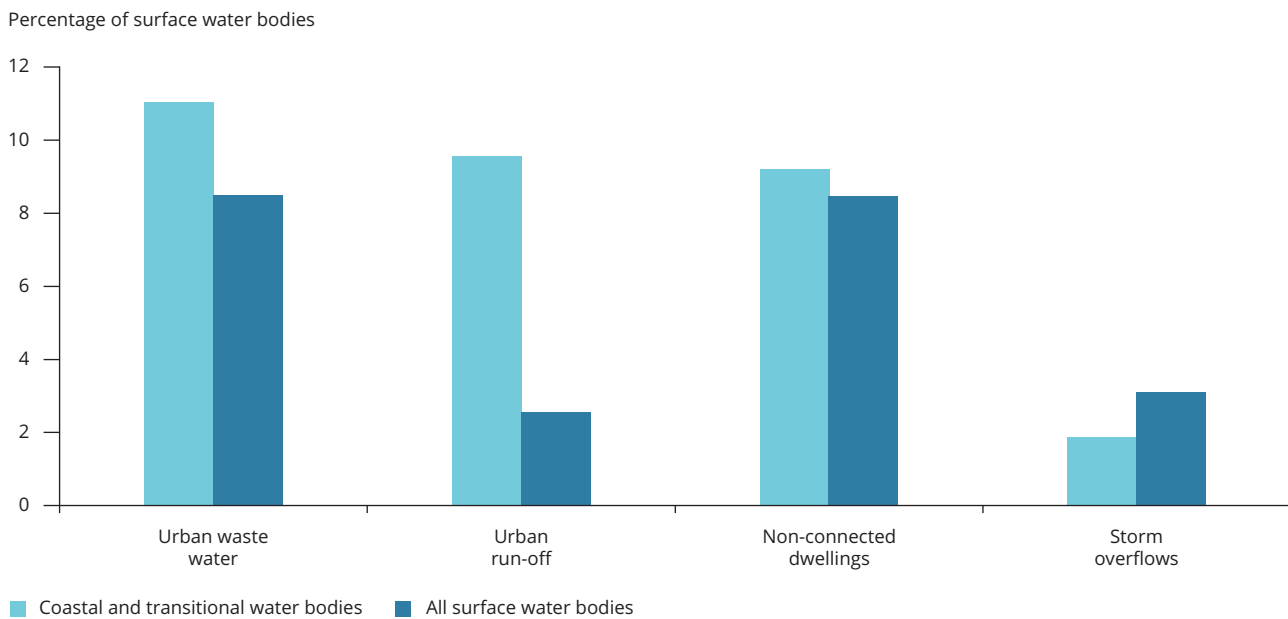
Figure 2.6 Selected significant pressures causing failure to achieve good ecological status (under second river basin management plans)
