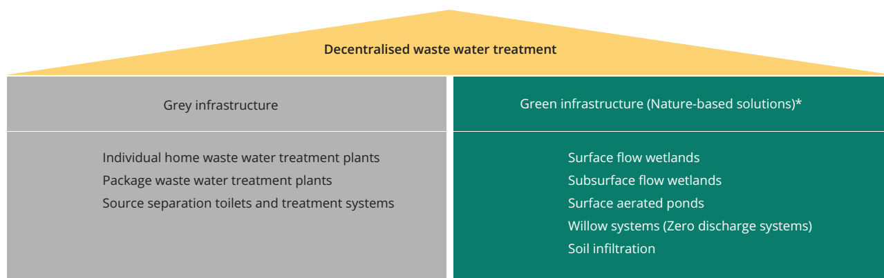
Figure 4.2 Decentralised sewage treatment
