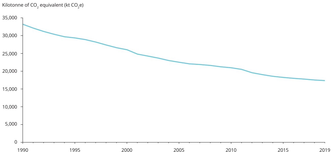
Figure 2.8 CO 2 e released by the domestic waste water treatment sector in the EU-27
