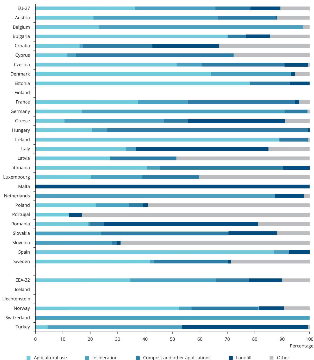
Figure 3.2 Sewage sludge management approaches in Europe
